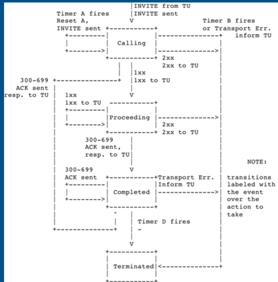
Figure 5: INVITE client transaction
